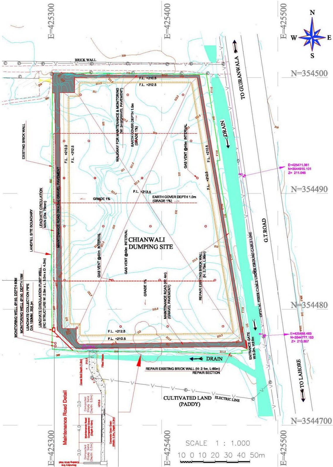
Figure 6.3.5 Layout Plan of Safe Closure Work at Chianwali Former Disposal Site
